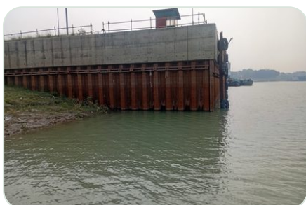
Cofferdam & sheet-pile works
